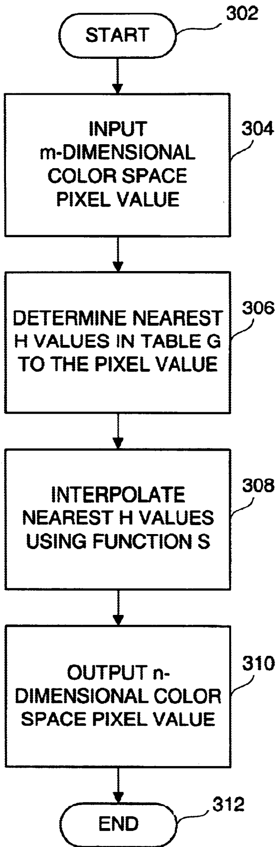
FIG. 3 TRANSFORMATION ROUTINE 300
